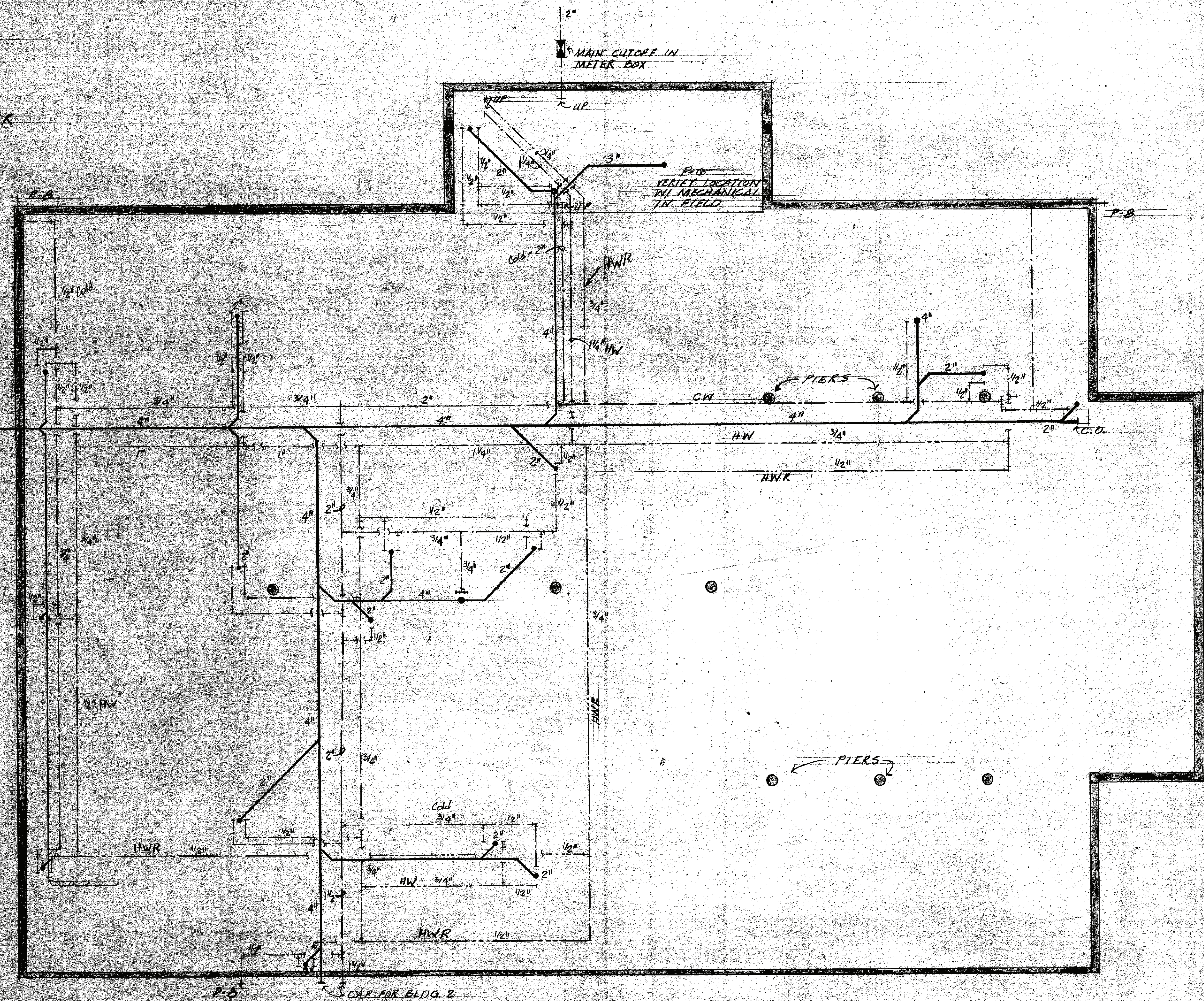
Foundation Sewer & Water Piping Plan Original Design, Initial (Front of Building Only) Provided for Information only
