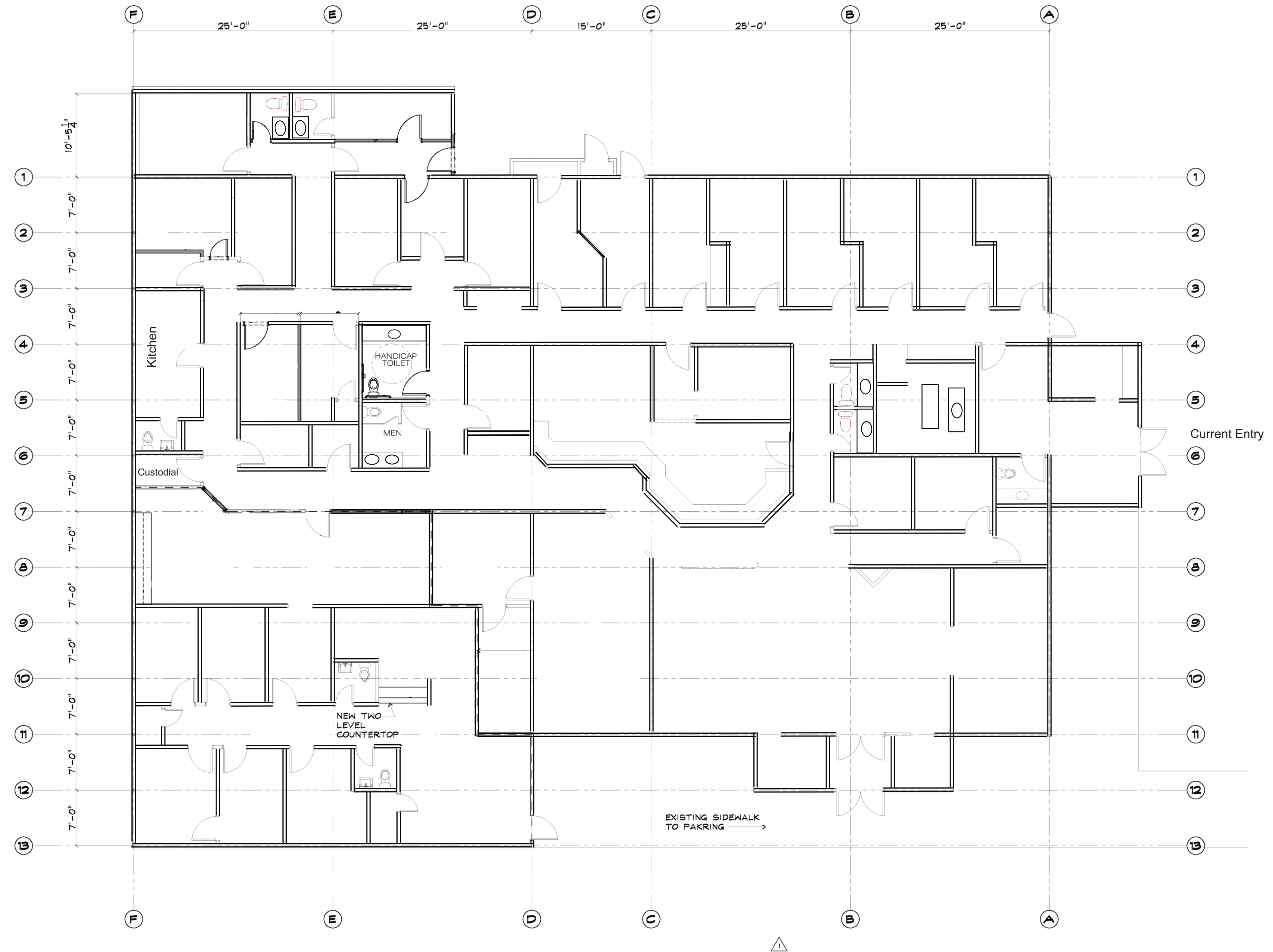
A A101 FLOOR PLAN SCALE 1/8" = 1'-0"
