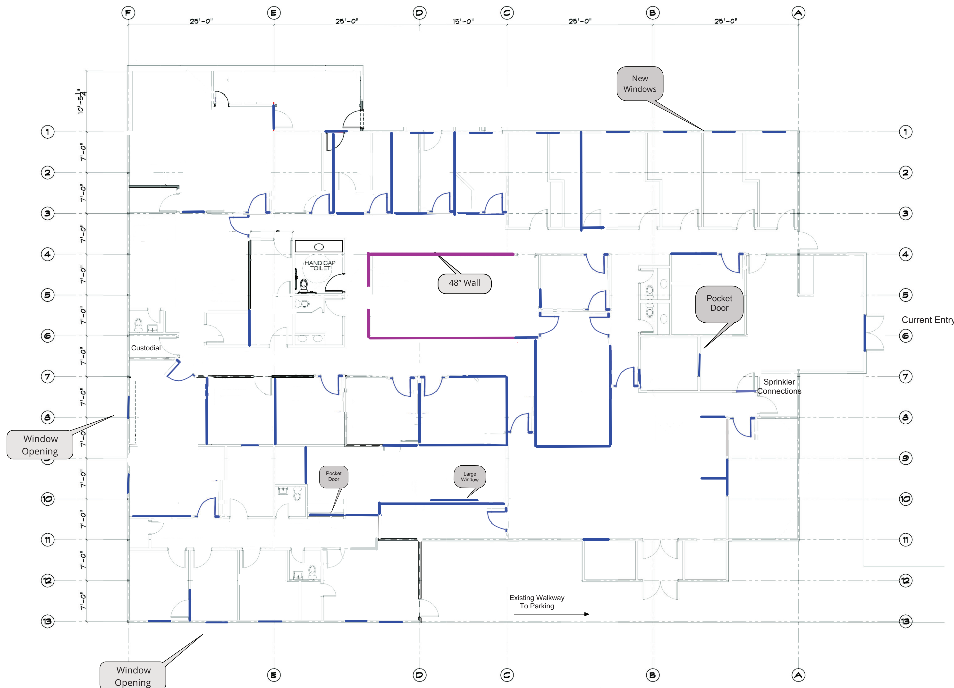
A101 FLOOR PLAN SCALE 1/8" = 1'-0"
